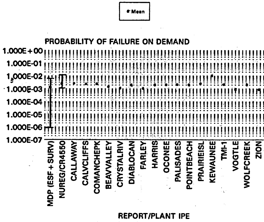
PWR CCW SYSTEM MDP PROBABILITY OF FAILURE ON DEMAND COMPARISON WITH VALUES USED IN IPEs FIGURE 6
