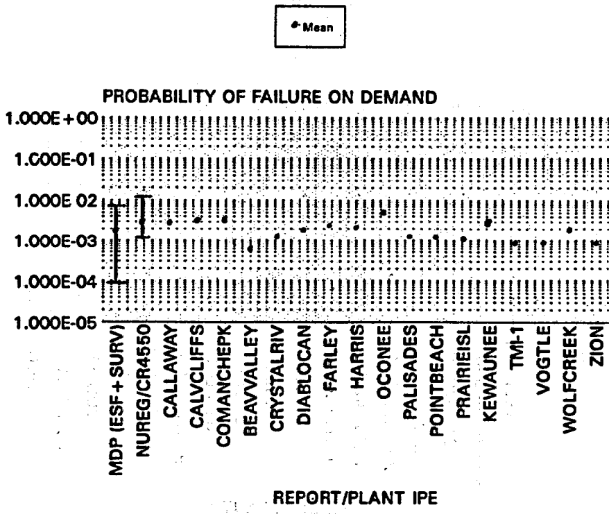
PWR CS SYSTEM MDP PROBABILITY OF FAILURE ON DEMAND COMPARISON WITH VALUES USED IN IPEs FIGURE 7
