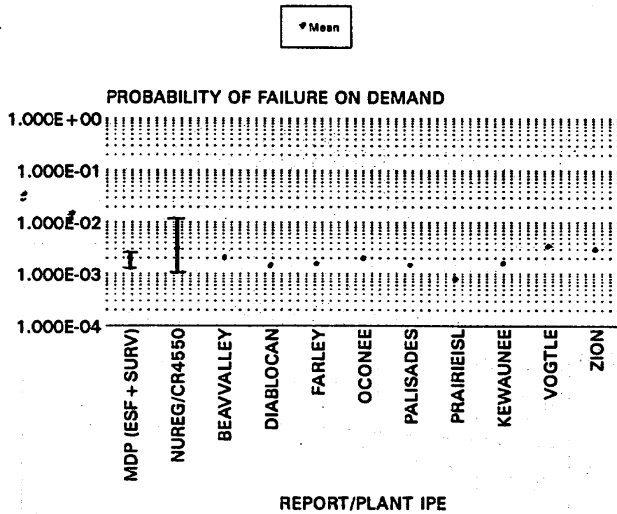
PWR AFW SYSTEM MDP PROBABILITY OF FAILURE ON DEMAND COMPARISON WITH VALUES USED IN IPEs
