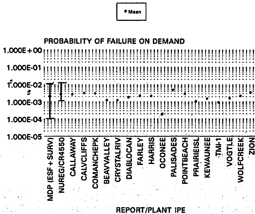
PWR HPI SYSTEM MDP PROBABILITY OF FAILURE ON DEMAND COMPARISON WITH VALUES USED IN IPEs
